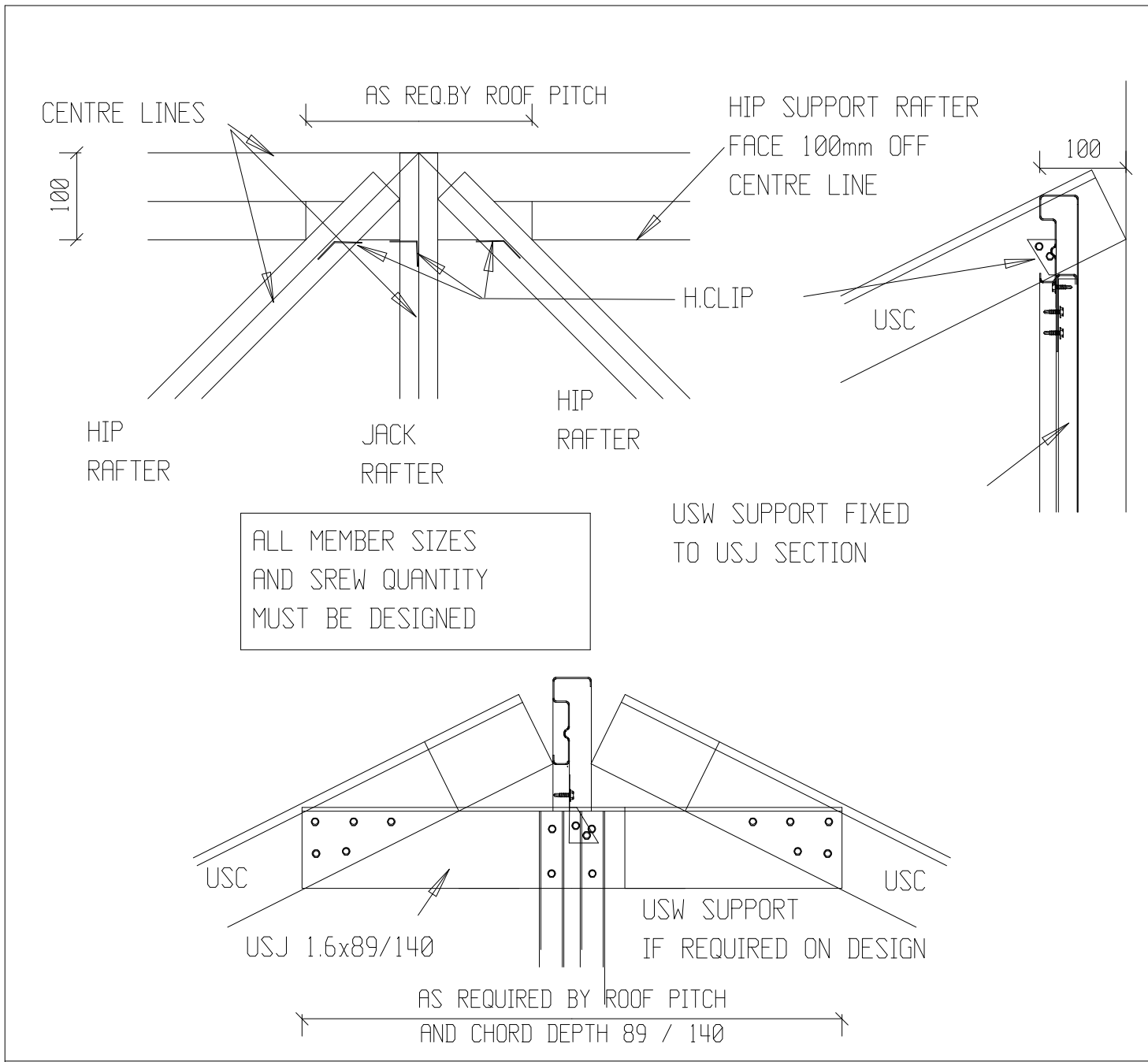
DETAIL - HIPAPEX
